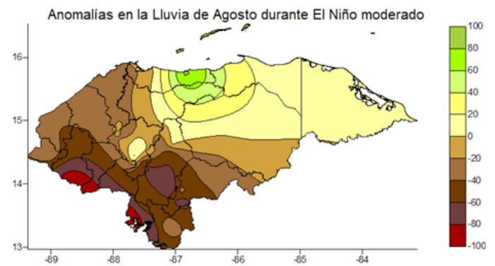
Figure 6. Rainfall anomalies during moderate El Niño events (originally published in Argeñal, 2010b)
