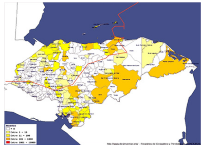
Figure 17. Trajectory of Hurricane Mitch and associated casualties by municipality (originally published in Kawas and Elvir Ferman, 2011a)
