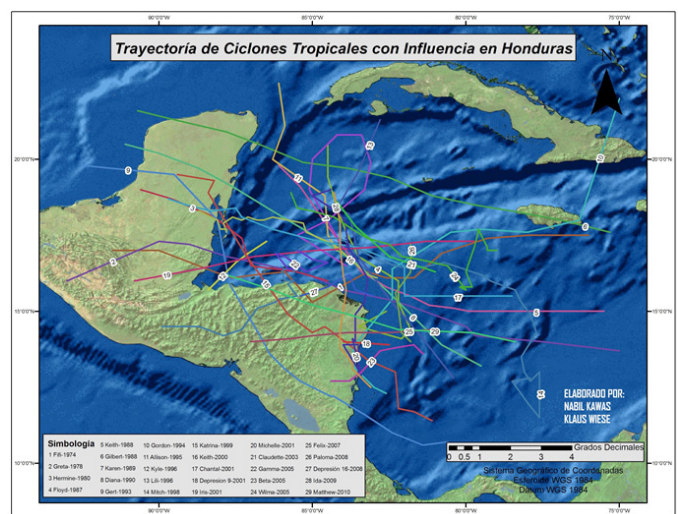
Figures 7 and 8. Pathways and hazard maps of tropical cyclones (originally published in Argeñal, 2010b)
