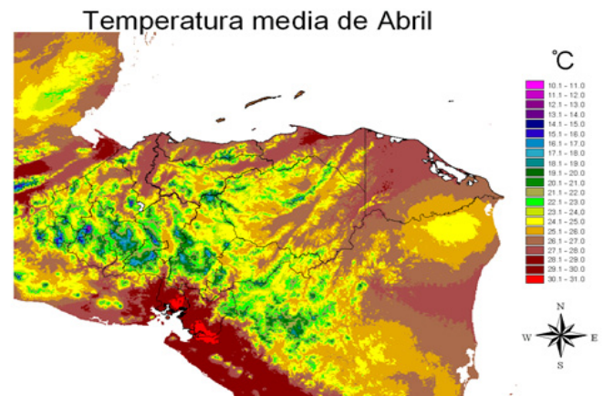
Figure 5. April mean temperatures (originally published in Argeñal, 2010b)
